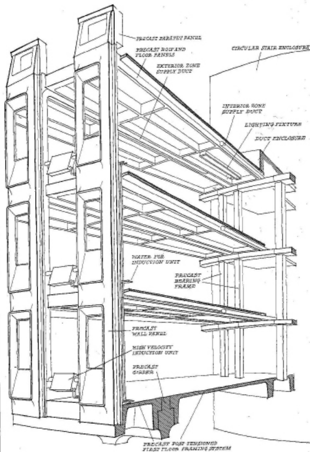
Figure 26. Diagram showing the assembly of the precast concrete panels. "Circling in the Square," Architectural Forum 118.
